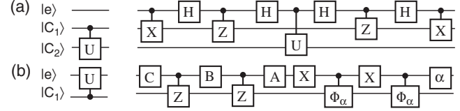
FIG. 2. Circuits for controlled gates U among two nuclear spins (a) and a nuclear and the electronic spin (b). The gates A , B , C are defined such that U = e^{i\alpha}AZBZC and ABC = \mathbb{1} , where Z is a \pi rotation around z [35]. \Phi_\alpha is a phase gate: |0\rangle \times \langle 0| + |1\rangle \langle 1| e^{i\alpha/2} and the gate \alpha indicates e^{i\alpha/2} \mathbb{1} .
