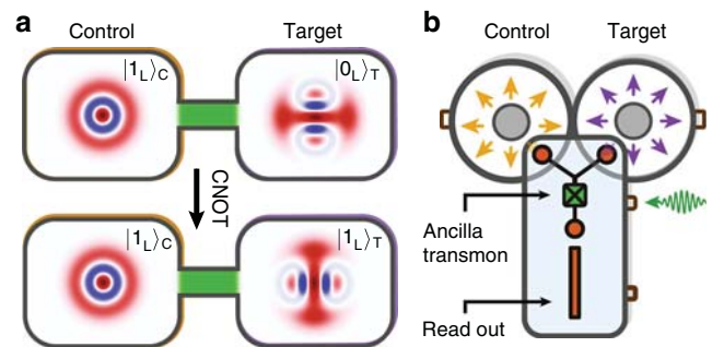
Fig. 1 Experimental implementation of an entangling gate between multiphoton qubits encoded in two cavities. a Example of the CNOT operation. In the initial state, illustrated by the Wigner distributions in the top panel, the control qubit is in |1_L\rangle_C , and the target qubit in |0_L\rangle_T (as defined in Eqs. (1) and (2)). Under the action of the CNOT gate, enabled by a nonlinear coupling between the cavities (in green), the target state at the output (bottom panel) is inverted to |1_L\rangle_T . b Sketch of the device, which is housed inside an aluminum box, and cooled down to 20 mK. The control and target qubits are encoded in photon states of the fundamental modes (yellow and purple arrows) of two coaxial cavities with frequencies \omega_C/2\pi = 4.22 GHz and \omega_T/2\pi = 5.45 GHz, respectively. The ancilla transmon ( \omega_q/2\pi = 4.79 GHz) has two coupling pads (orange circles) that overlap with the cavity fields. Cavity-ancilla interaction is achieved by application of a frequency-matched RF drive (green arrow) to the coupling pin near the Josephson junction (marked by X). The ancilla also serves to prepare and read out the cavity state, and is measured by its dispersive coupling to a stripline readout resonator (orange rectangle). More details on this device can be found in Supplementary Note 1 and ref. 20
