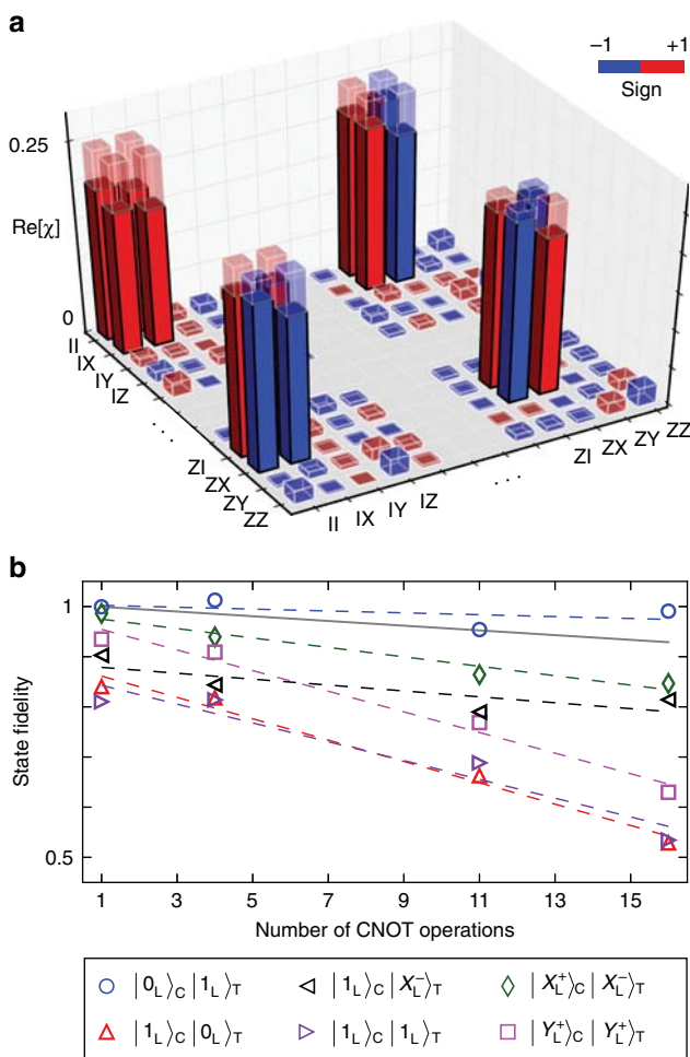
Fig. 4 Characterization of the controlled NOT gate. a Quantum process tomography. The solid (transparent) bars represent the measured (ideal) elements of the process matrix \chi . The corresponding process fidelity is F_{\text{CNOT}} = (89 \pm 2)\% . For clarity, only the corners of the process matrix are presented. The full \chi -matrix is shown in Supplementary Note 8 for completeness. b State fidelity under repeated gate applications for various input states, chosen to highlight different error mechanisms of the gate (the dashed lines are linear fits). The solid gray line depicts the simulated average slope of state fidelity imposed by ancilla decoherence. The state fidelities are calibrated by the value measured for the vacuum state (Supplementary Note 6). The standard errors are derived from bootstrapping, and are equal in size to the symbols
