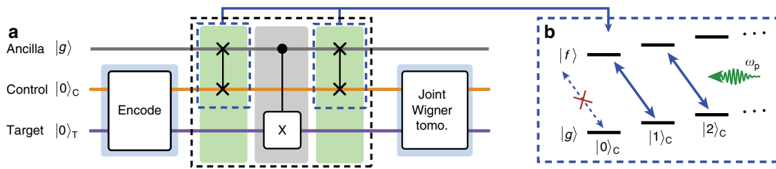
Fig. 2 Protocol of the entangling gate. a The sequence starts with preparation of the desired initial two-cavity state, while leaving the ancilla transmon in the ground state. The cavity-cavity CNOT gate (dashed black rectangle) consists of two entangling gates between the control cavity and the ancilla (dashed blue rectangles), interleaved by a CNOT gate between the ancilla and the target, implemented by a conditional \pi/2 phase-space rotation of the target cavity. The joint Wigner distribution of the final two-cavity state is measured using a method similar to ref. 20 . b Schematic level diagram illustrating the RF-driven control-ancilla sideband transition. Through the absorption of a single drive photon (in green) and a single control photon, the ancilla is doubly excited from |g\rangle to |f\rangle (solid blue arrows). However, when the control cavity is in vacuum, the absence of a control photon prevents the ancilla from being excited to |f\rangle (dashed blue arrow)
