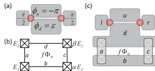
FIG. 1 (color online). On the surface of the TI, patterned SC islands can form (a) STIS quantum wire, (b) flux qubit, and (c) a hybrid system of topological and flux qubits. (a) Two MFs (red dots) are localized at two SC trijunctions, connected by an STIS quantum wire (dashed blue line). The coupling between the MFs is controlled by the SC phases \phi_d = \epsilon and \phi_u = -\pi . (b) A flux qubit consists of four JJs connecting four SC islands ( a, b, c, d ) in series, enclosing an external magnetic flux f\Phi_0 . (c) The hybrid system consists of an STIS wire and a flux qubit. The STIS wire (between islands d and u ) couples the MFs, with coupling strength controlled by the flux qubit. The SC phase \phi_c can be tuned by a phase controller (not shown), and \phi_d = \phi_c \pm \theta_4^* with the choice of \pm sign depending on the state of the flux qubit.
